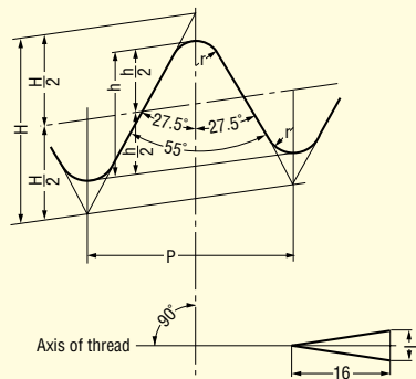
Basic Profile Applied for Taper External and Taper Internal Threads
