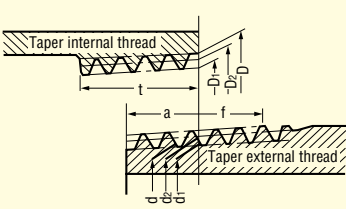
How to Symbolize taper pipe threads :
