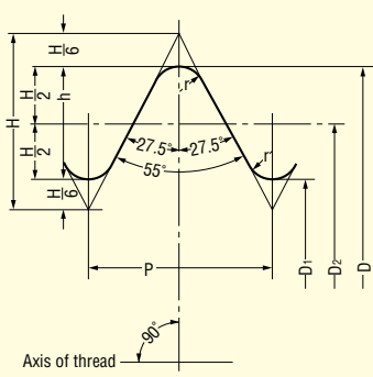
Basic Profile Applied for Parallel Internal Threads
