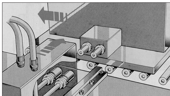
▲ Oil and air circuits connect/disconnect automatically for automatic mold replacement
