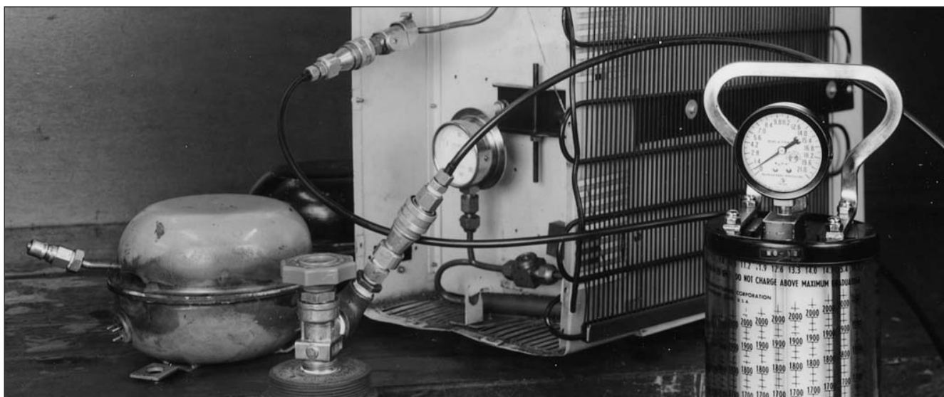
▲ Vacuum extraction
