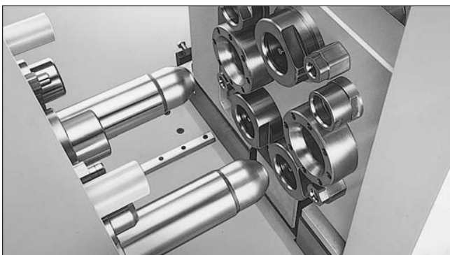
▲ Multiple pipes
